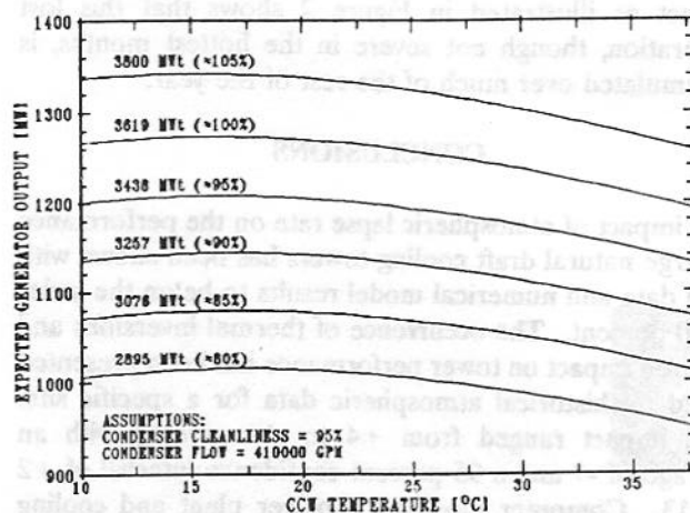
Figure 3. Generator Output for BLN vs. CCW Inlet Temperature
